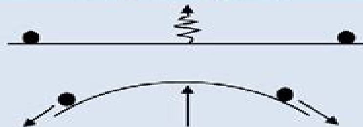
Repulsion negative gravity
