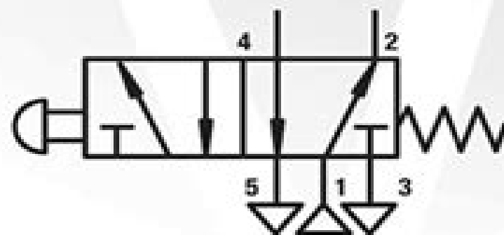
5/2 valve
