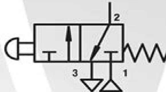
3/2 valve
