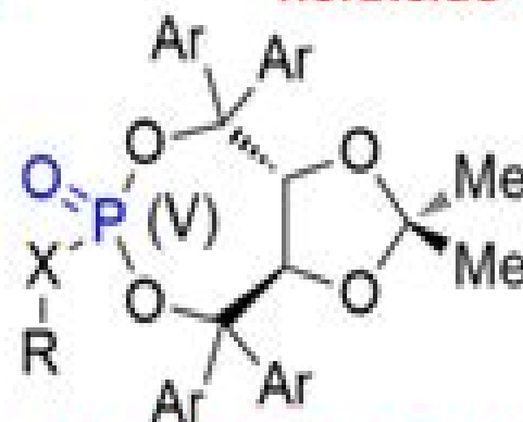
axially chiral phosphorus: catalysts and ligands
