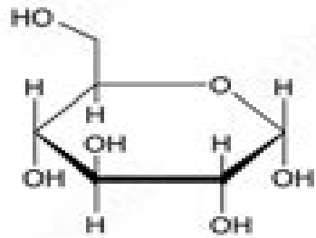
Alpha-D-Glucose
