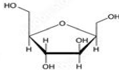
Alpha-D-Fructose
