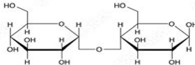
Maltose
