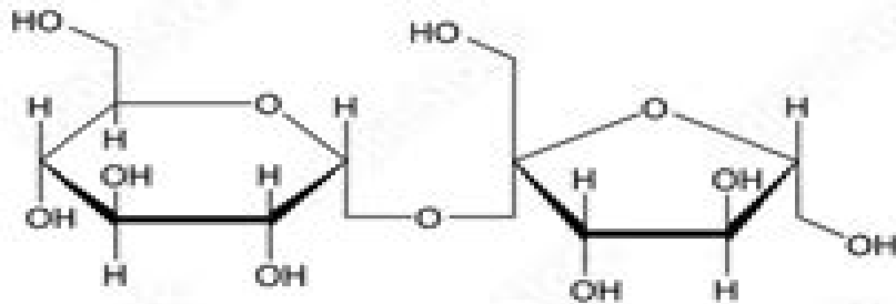
Sucrose (saccharose)
