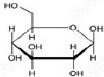
Beta-D-Glucose
