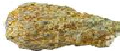
pyrite
