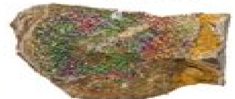
rainbow pyrite
