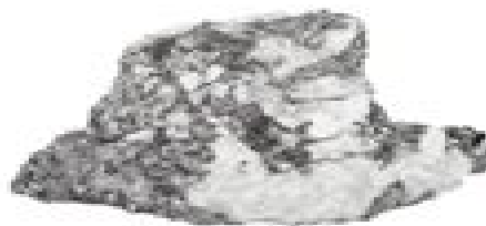
bismuthinite
