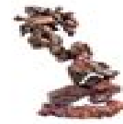
native copper
