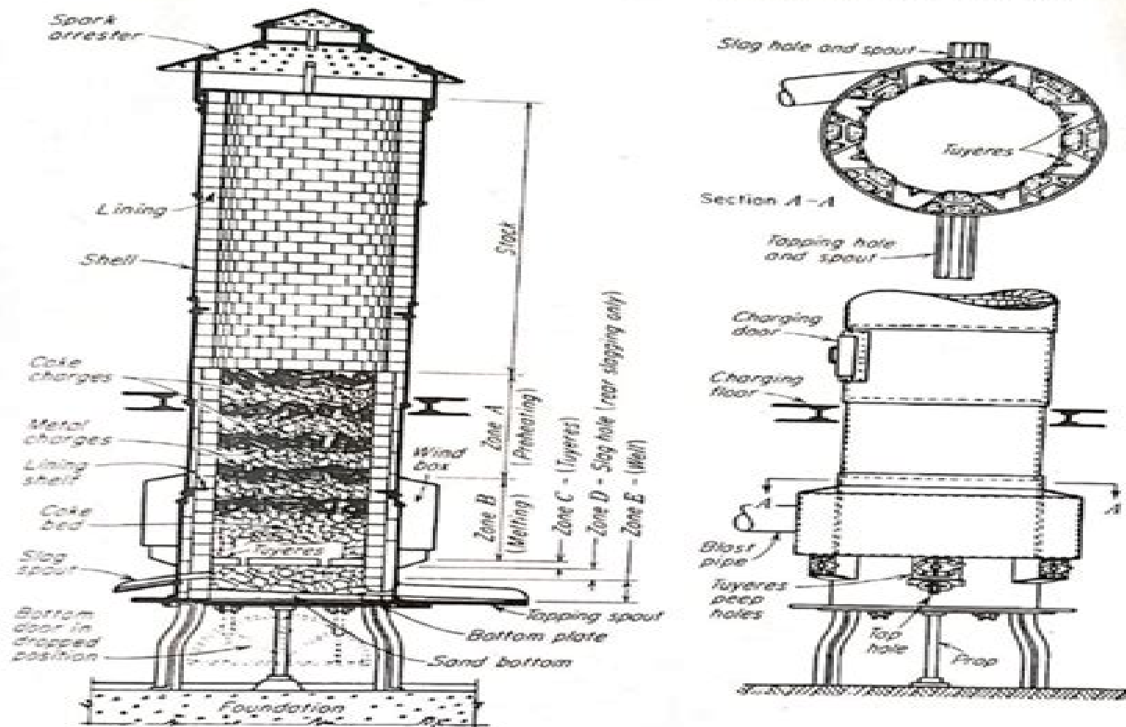
Fig. 19.1 Structure of the common cupola. (From American Foundrymen's Society .)
