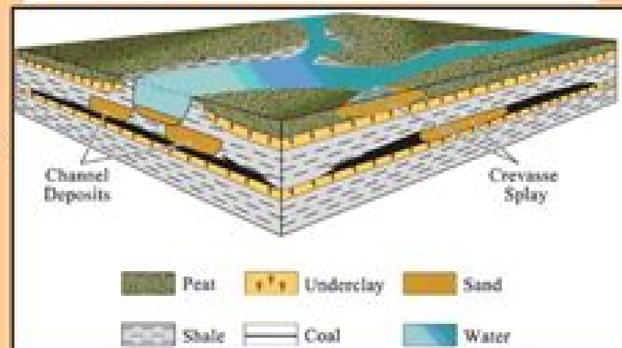
Example of sedimentary facies model: Delta distributary channel
