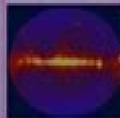
gamma rays
