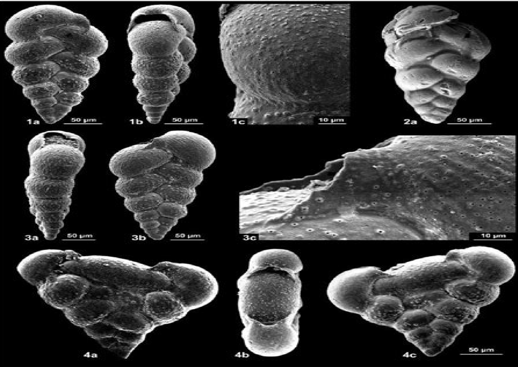
Figure 8. Hypotypes and a paratype of Loxitherohelix pulchra (Brøtzen, 1936) and a hypotype of Loxitherohelix reniformis (Marie, 1941). Planctic foraminiferal zonation after Georgescu (2006) (1) and Huber (1992), Huber et al. (1995) (3–4). 1a–1b: Hypotype from the upper Campanian ( Radiotruncana calcarata Biozone) of the Marshalltown Formation, New Jersey coastal plain (ODP Leg 174AN, Bass River Site), Sample 433.59–.60 m. 2a: Paratype from the lower Senonian (Erikodal, Sweden) deposited at the National Museum of Natural History, Smithsonian Institution (USNM 307972), Washington, D.C. 3a–3c: Specimen from the lower Campanian ( Archaeoglobigerina cretacea Biozone) of the Falkland Plateau (South Atlantic), Sample 79-511-31-5, 33–35 cm. 4a–4b: Hypotype of Loxitherohelix reniformis from the upper lower Campanian ( Archaeoglobigerina cretacea Biozone), Sample 511-32-CC. (specimen previously figured by Georgescu et al. , 2009, pl. 2, figs. D1–3).
