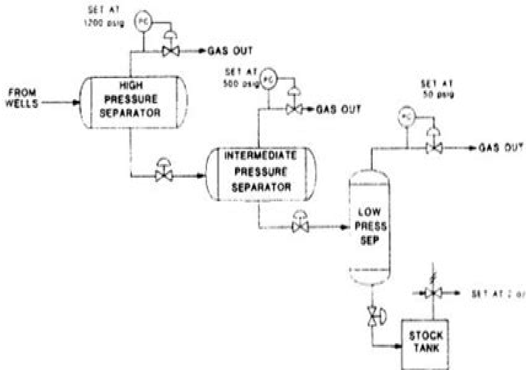
Figure 6-1. Multistage separation process.
