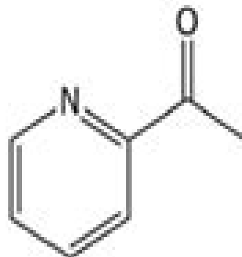
2-Acetylpyridine [14.038]
