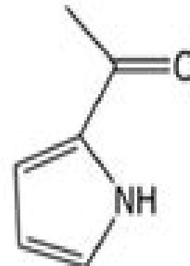
2-Acetylpyrrole [14.047]
