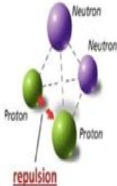
Electric Forces
