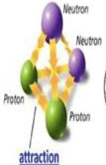
Strong Nuclear Forces
