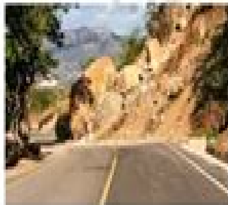
Landslide
