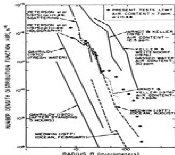
FIGURE 43. Nuclei distributions from various sources.
