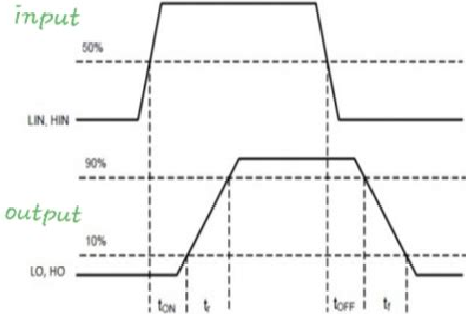
Figure 4. Propagation Delay, Rise and Fall Times
