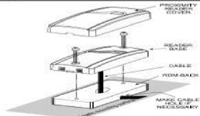
Figure 3. RDM-4 Mounting
