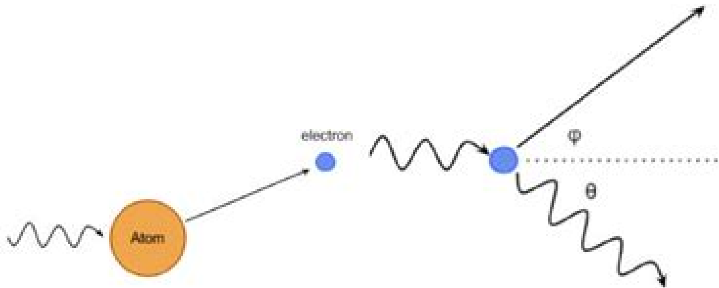
(a) Photoelectric Effect
