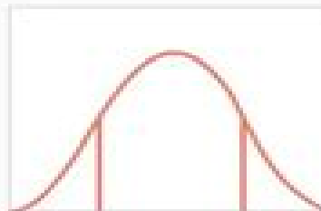
T-test distribution
