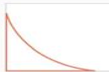
Exponential distribution
