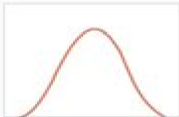
Normal distribution
