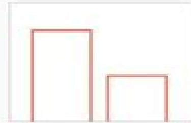
Bernoulli distribution
