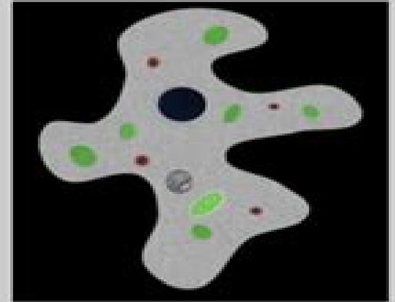
Amoeba
