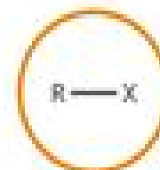
HALOALKANE
