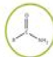
AMIDE
