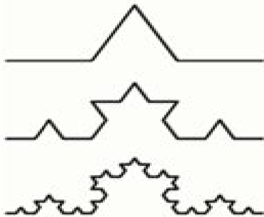
Koch curve
