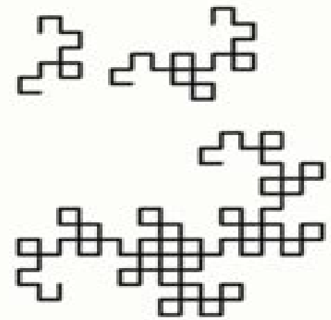
Dragon curve
