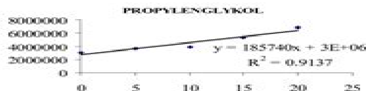
Fig. 2. Linear regression analysis shows dependence of average area on the volume of the stock reference compound mixture for 1,2-propanediol
