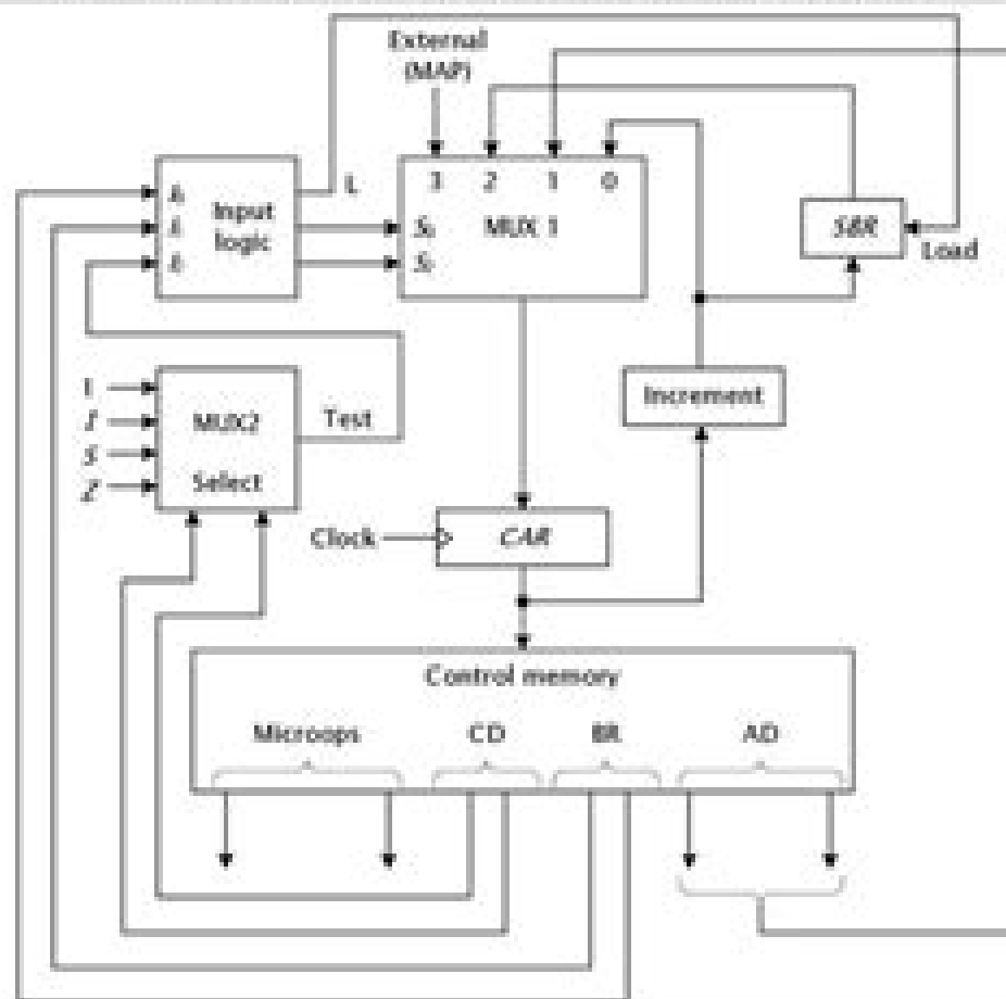
Fig. 7-8 Mircoprogram sequence for a control memory
