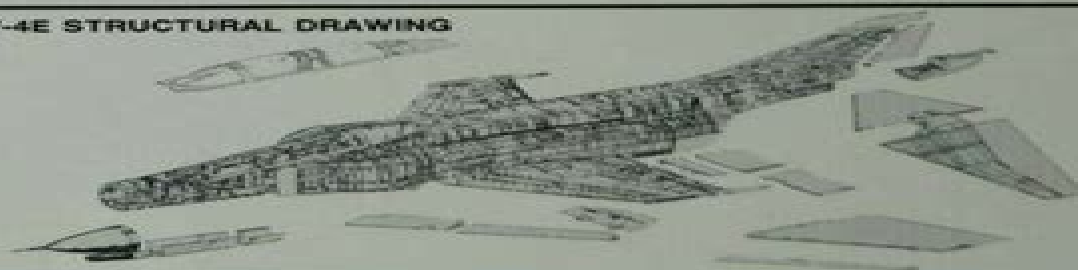
F-4E STRUCTURAL DRAWING
