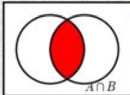
Intersection of two sets
