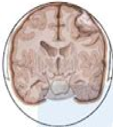
Meningioma Tumors
