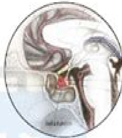
Pituitary Adenomas
