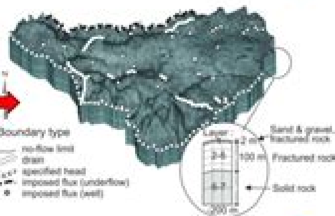
Hydrogeological model
