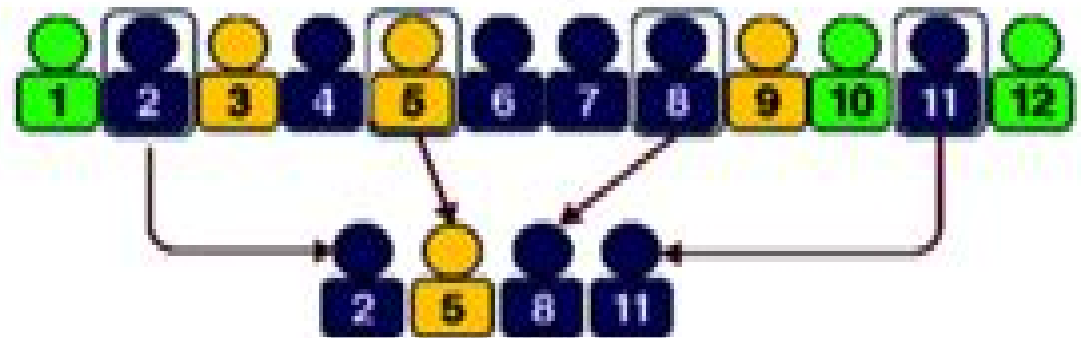
Systematic Sampling
