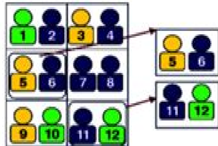
Clustered Sampling
