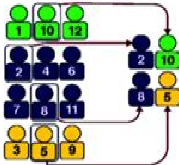
Stratified Sampling
