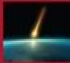
Meteorite
