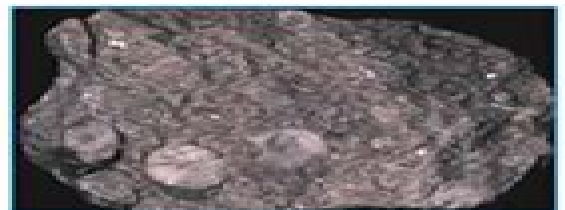
38. Crinoidal limestone
