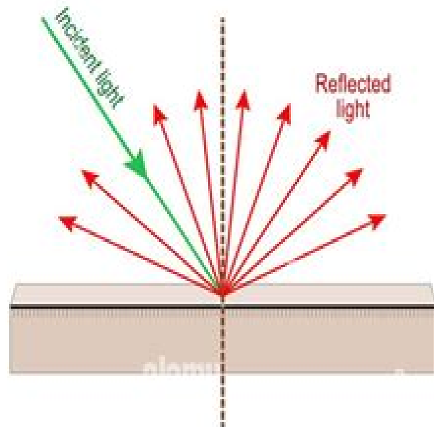
Diffuse reflection
