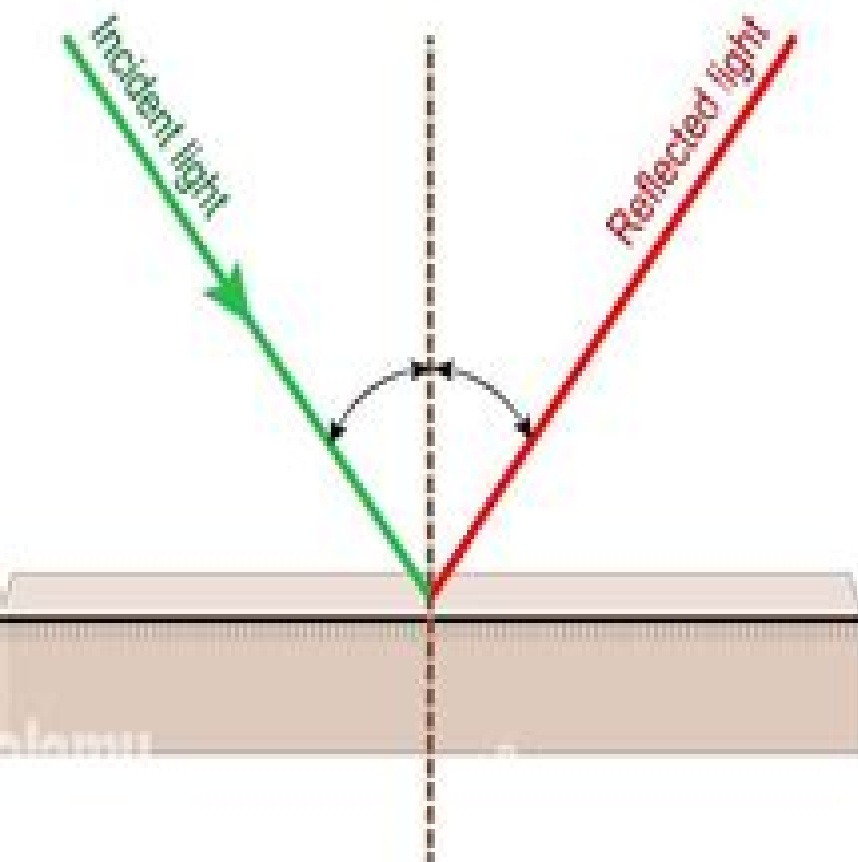
Specular reflection
