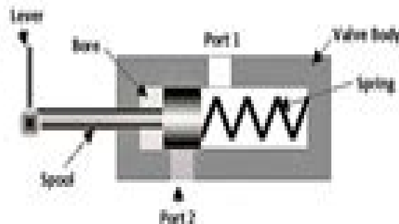
2-way Direction Control Valve
