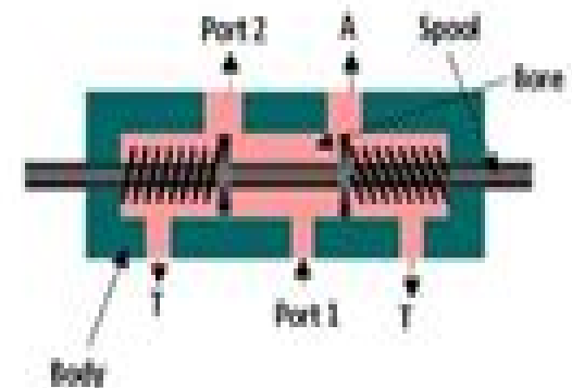
4-way Direction Control Valve
