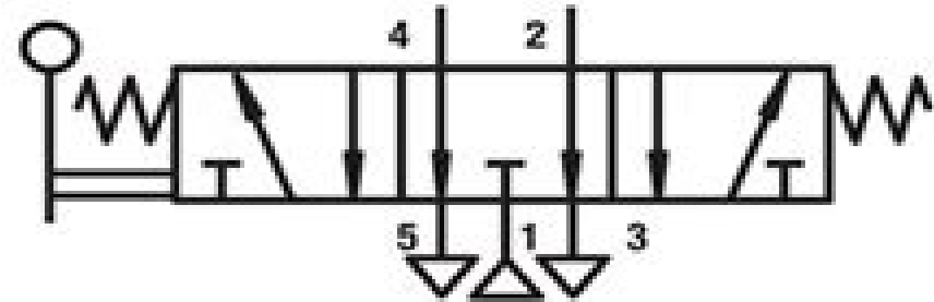
5/3 valve, supply port only sealed
