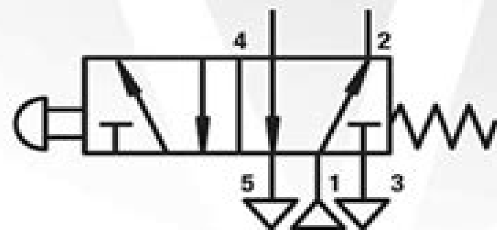
5/2 valve
