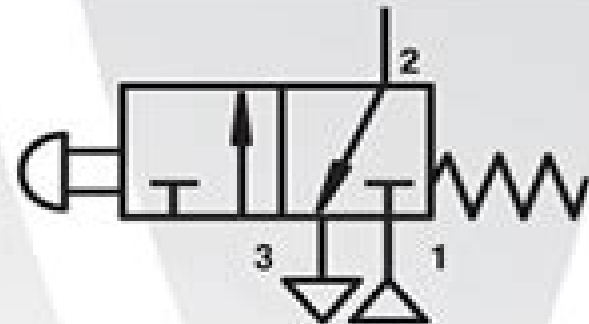
3/2 valve
