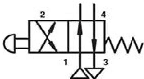
4/2 valve
