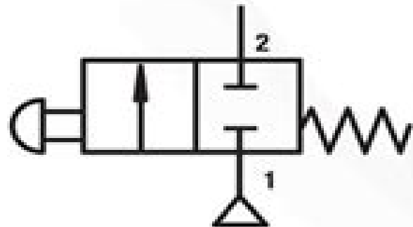
2/2 valve
