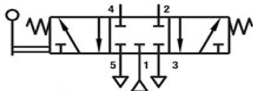
5/3 valve, all ports sealed
