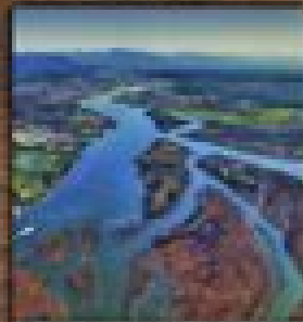
delta
