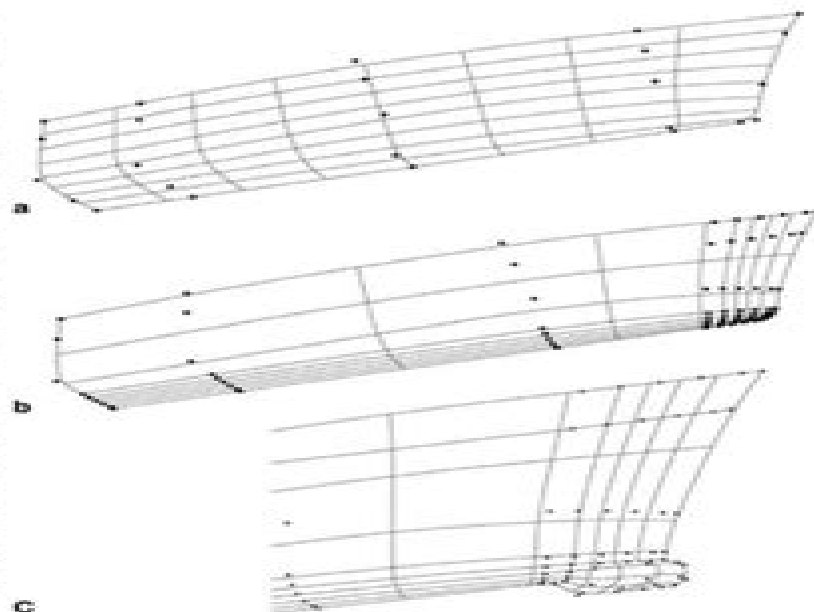
Fig. 40 Sonar dome at the forefoot of a hull, formed as an integral part of the B-spline hull surface by addition of rows and columns of control points.
