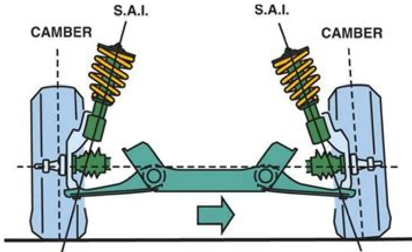
FIGURE 17-40 Cradle placement. If the cradle is not replaced in the exact position after removal for a transmission or clutch replacement, the SAI, camber, and included angle will not be equal side-to-side.
