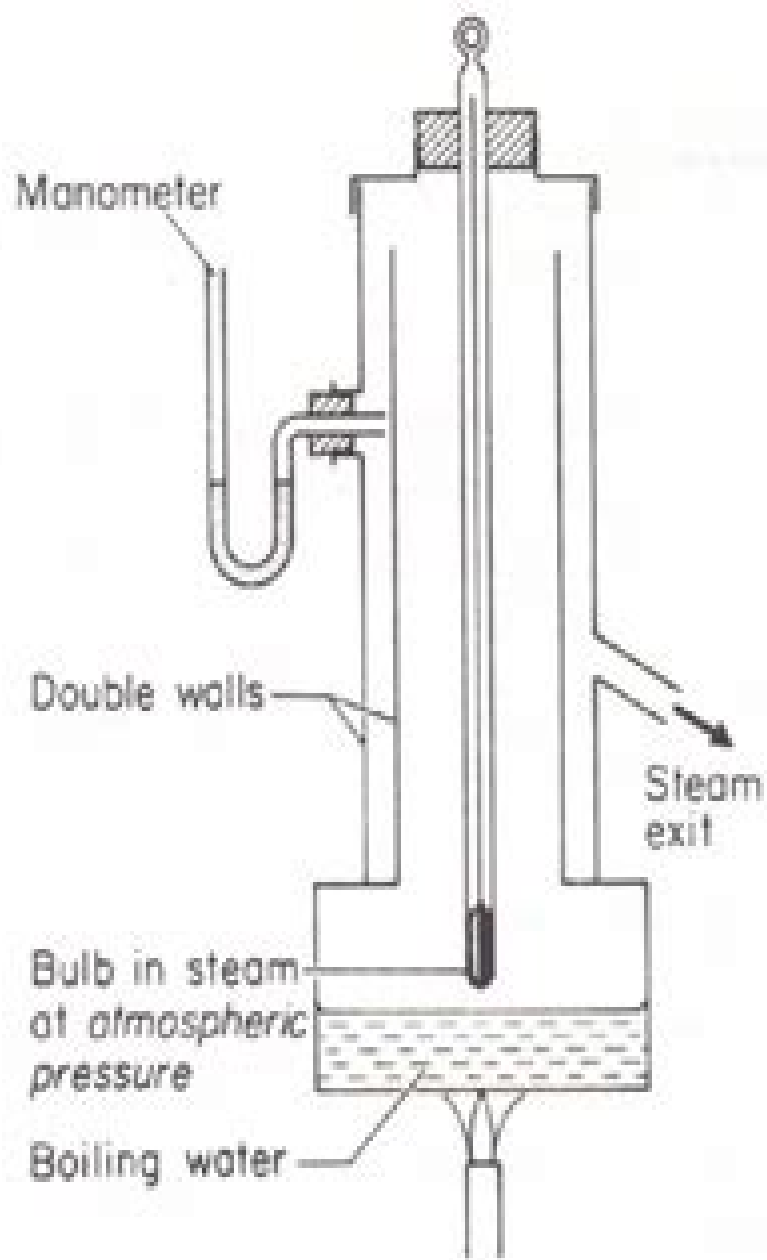
Fig. 14.2. Hypsometer (upper fixed point)
