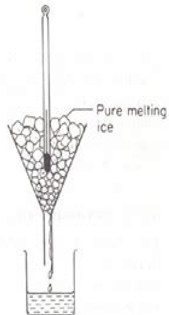
Fig. 14.3. Lower fixed point
