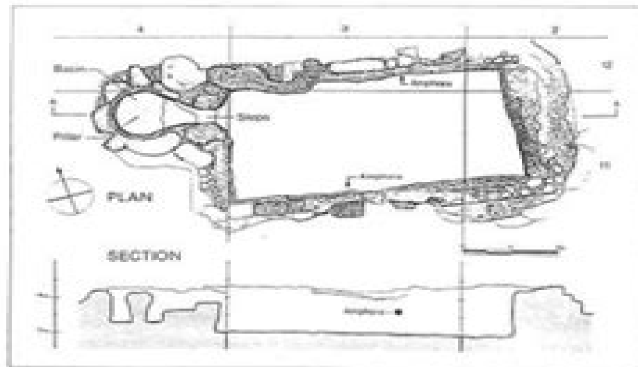
FIGURE 105. Paestum, Santa Venera — plan and section of the fishpond. (Drawing by David Myers)
