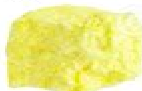
sulphur
