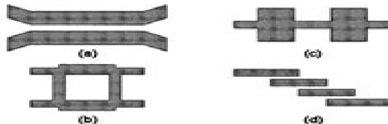
Fig. 2. Stripline-components. (a) TEM-line proximity coupler. (b) Branch-line coupler. (c) Low-pass filter. (d) Bandpass filter.
