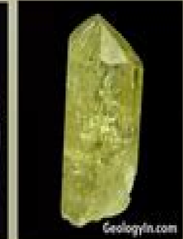
Phosphates - Apatite
