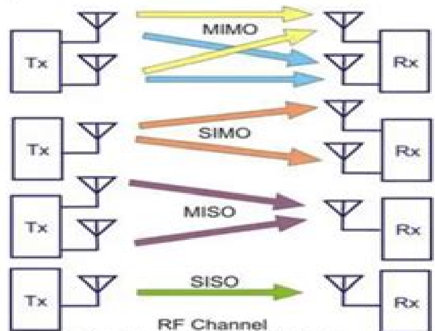
Figure 1: Typical MIMO System
