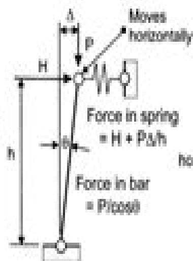
(b) P-\Delta
