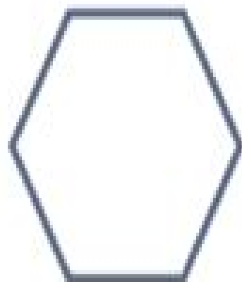
hexagon
