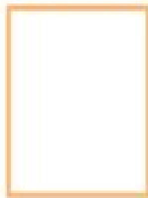
square
