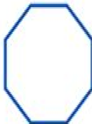
octagon
