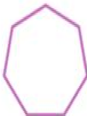
heptagon
