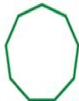
nonagon
