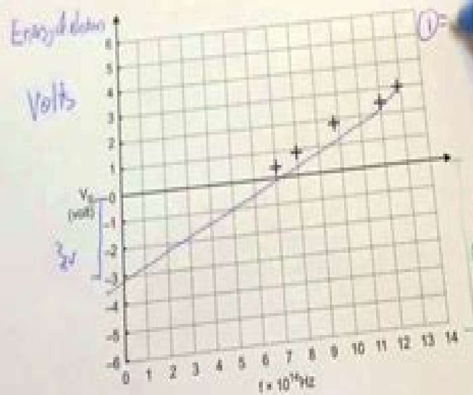
Figure 3 shows the stopping voltage, V_0 , as a function of the frequency ( f ) of the light falling on the plate.
