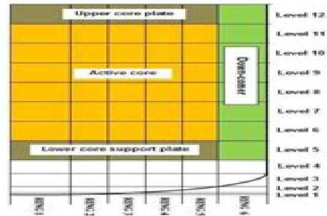
Fig. 2. A nodalization scheme for structures in reactor core, lower plenum and downcomer
