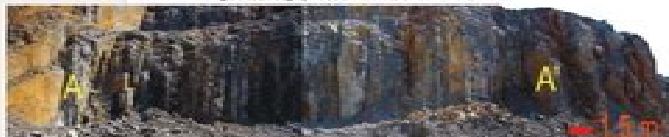
Figure 3. Field views of K-bentonites at limestone quarries excavated in Yılanı formation
