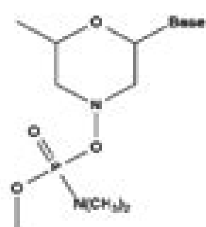
Morpholino phosphoramidate
