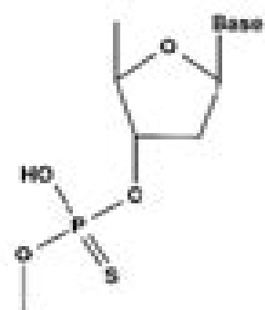
Phosphorothioate
