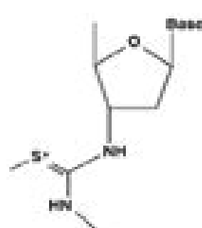
S-methylthiourea
