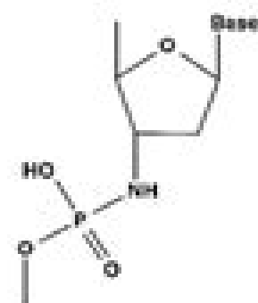
Phosphoramidate
