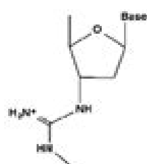
Guanidinium
