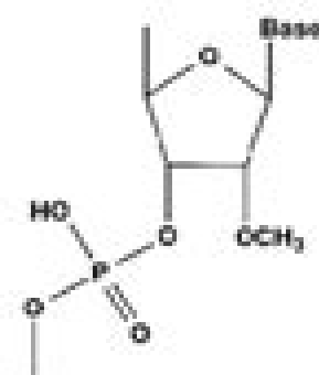
2'-O-Methyl
