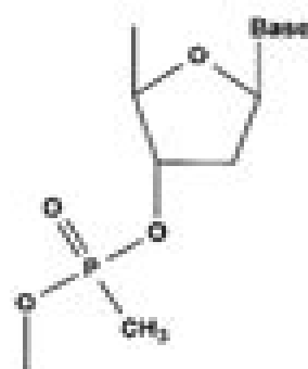
Methylphosphonate
