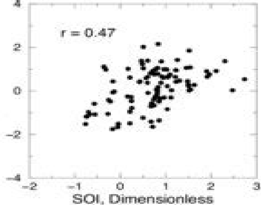
(b) 1960–84 SOI vs. Flow RPC 2
