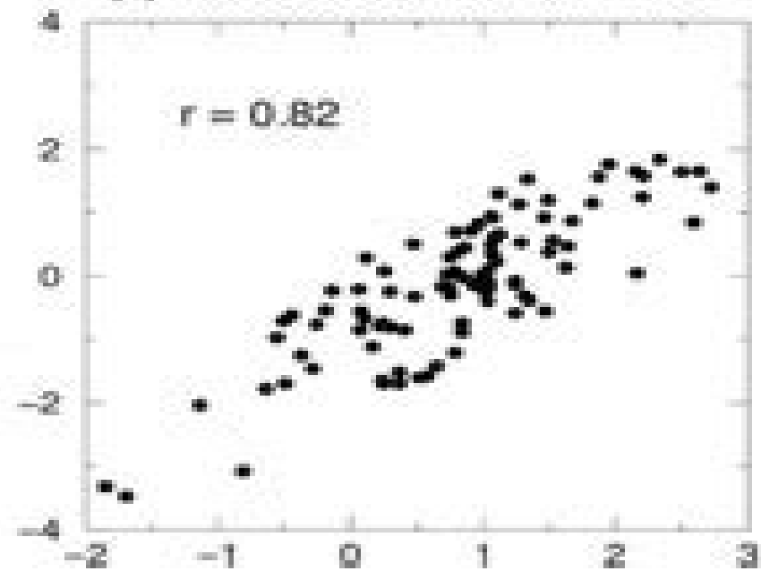
(b) 1960–84 SOI vs. Flow RPC 2
