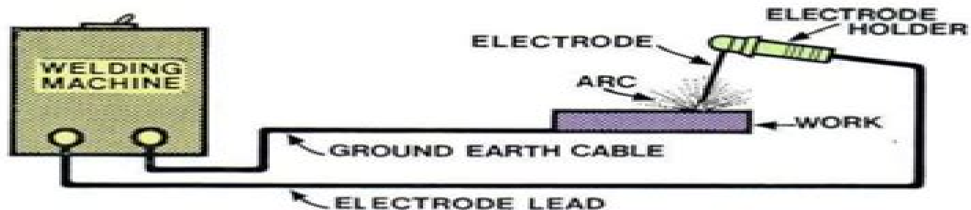
Figure 3.1: Arc welding set up.
